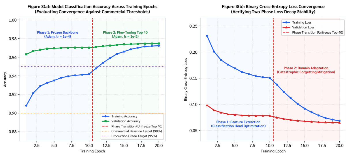
Two-phase Cloud GPU training history.
